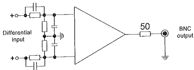
Differential probe principle
