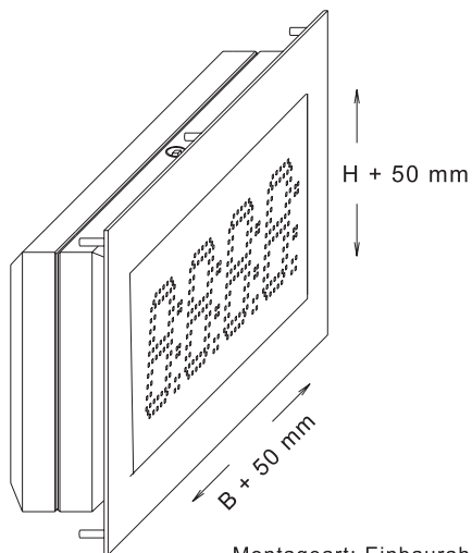
Montageart: Einbaurahmen Mounting: mounting frame
